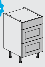
500 3 Drawer Cabinet 720mm H x 500mm W x 570mm D
