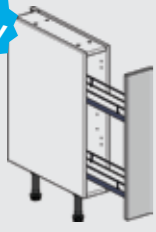
150 Base Pull-Out Cabinet 720mm H x 150mm W x 570mm D
