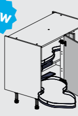
1000 Blind Corner w/ LH Nuvola Pull-Out 720mm H x 1000mm W x 570mm D | Planning Dimensions 1150mm x 650mm
