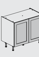
1000 Base Cabinet 720mm H x 1000mm W x 570mm D
