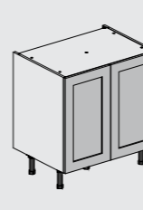
800 Base Cabinet 720mm H x 800mm W x 570mm D
