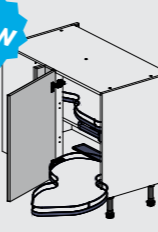
1000 Blind Corner w/ RH Nuvola Pull-Out 720mm H x 1000mm W x 570mm D | Planning Dimensions 1150mm x 650mm
