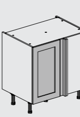
800 Blind Corner 720mm H x 800mm W x 570mm D
